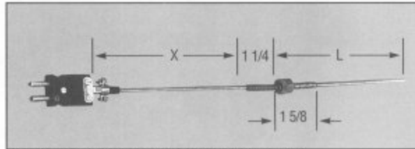
For Bayonet Adapter See Page 169 Catalog Number 1513
